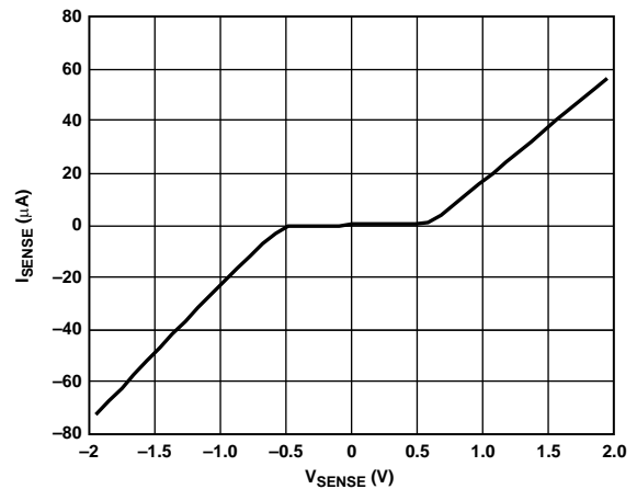
Figure 20. I SENSE vs. (V SENSE - V EE )
