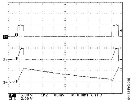
Figure 45. Timing Waveforms during a Retry Cycle for C_{TIMER} = 0.82\text{ nF} (Ch1 = GATE; Ch2 = SENSE; Ch3 = TIMER)
