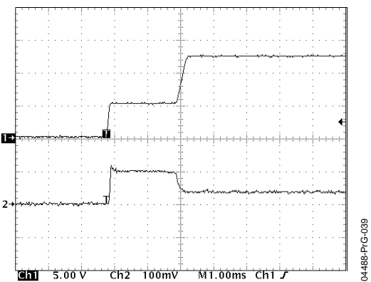
Figure 40. Soft Start Profile with a 0.1 nF Capacitor (Ch1 = GATE; Ch2 = SENSE)
